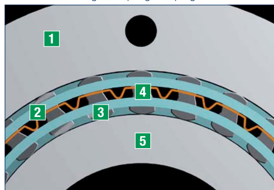
Torque transmission
