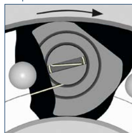
Torque transmission
